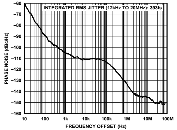
Figure 10. Absolute Phase Noise (Output Driver = HSTL), f_R = 19.44 \text{ MHz} , f_{OUT} = 644.53 \text{ MHz} , DPLL Loop BW = 0.1 Hz, f_{SYS} = 19.2 \text{ MHz} TCXO
