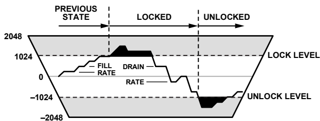
Figure 38. Lock Detector Diagram
