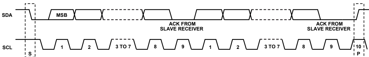
Figure 54. Acknowledge Bit
