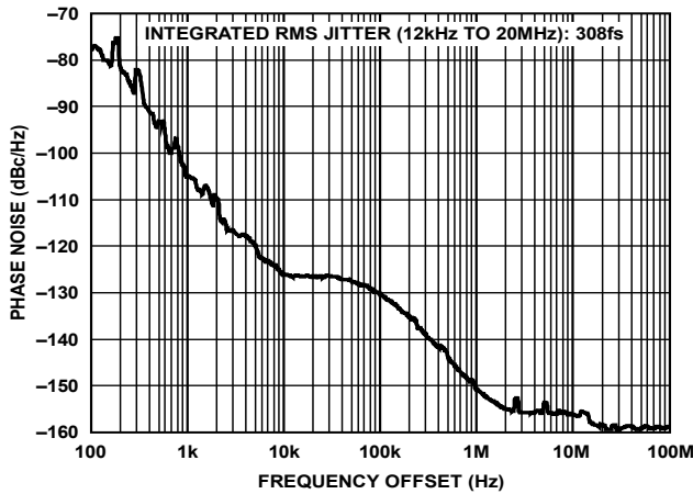
Figure 8. Absolute Phase Noise (Output Driver = HSTL), f_R = 2 \text{ kHz} , f_{OUT} = 125 \text{ MHz} , DPLL Loop BW = 100 Hz, f_{SYS} = 49.152 \text{ MHz} Crystal
