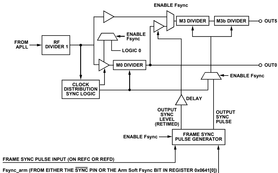
Figure 42. Frame Synchronization in One Shot Mode
