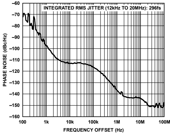
Figure 3. Absolute Phase Noise (Output Driver = HSTL), f_R = 19.44 MHz, f_{OUT} = 622.08 MHz, DPLL Loop BW = 50 Hz, f_{SYS} = 49.152 MHz Crystal
