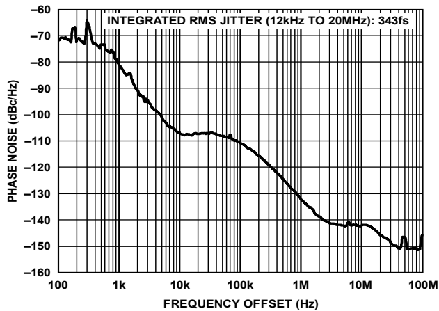
Figure 9. Absolute Phase Noise (Output Driver = HSTL), f_R = 25 \text{ MHz} , f_{OUT} = 1 \text{ GHz} , DPLL Loop BW = 500 Hz, f_{SYS} = 49.152 \text{ MHz} Crystal
