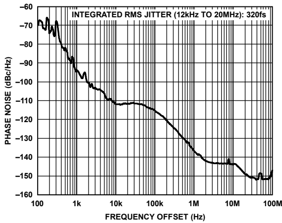
Figure 4. Absolute Phase Noise (Output Driver = HSTL), f_R = 19.44 MHz, f_{OUT} = 644.53125 MHz, DPLL Loop BW = 50 Hz, f_{SYS} = 49.152 MHz Crystal
