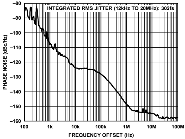
Figure 7. Absolute Phase Noise (Output Driver = 3.3V CMOS), f_R = 19.44 \text{ MHz} , f_{OUT} = 161.1328125 \text{ MHz} , DPLL Loop BW = 100 Hz, f_{SYS} = 49.152 \text{ MHz} Crystal
