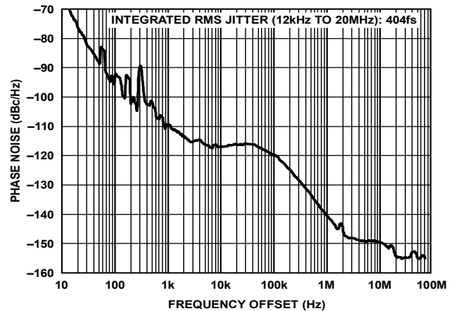
Figure 12. Absolute Phase Noise (Output Driver = HSTL), f_R = 19.44 \text{ MHz} , f_{OUT} = 312.5 \text{ MHz} , DPLL Loop BW = 0.1 Hz, f_{SYS} = 19.2 \text{ MHz} TCXO
