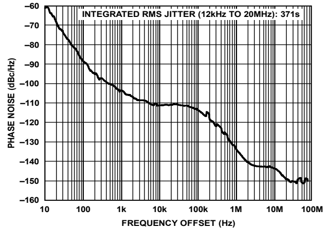
Figure 11. Absolute Phase Noise (Output Driver = HSTL), f_R = 19.44 \text{ MHz} , f_{OUT} = 693.482991 \text{ MHz} , DPLL Loop BW = 0.1 Hz, f_{SYS} = 19.2 \text{ MHz} TCXO
