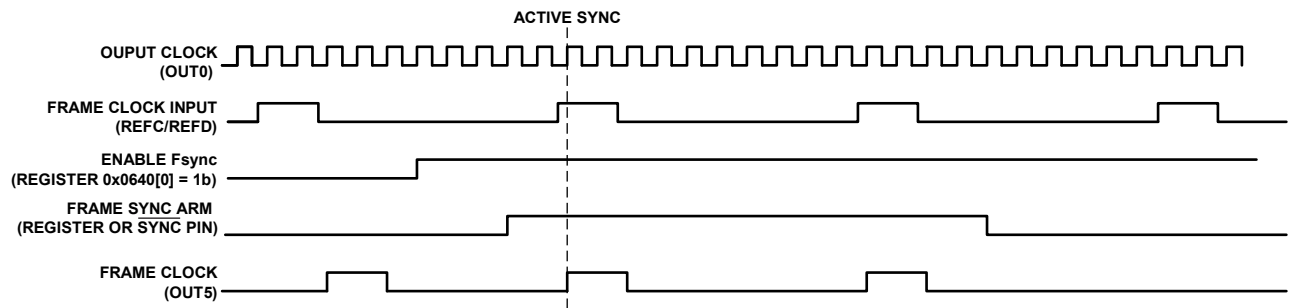
Figure 41. Frame Synchronization in Level Sensitive Mode
