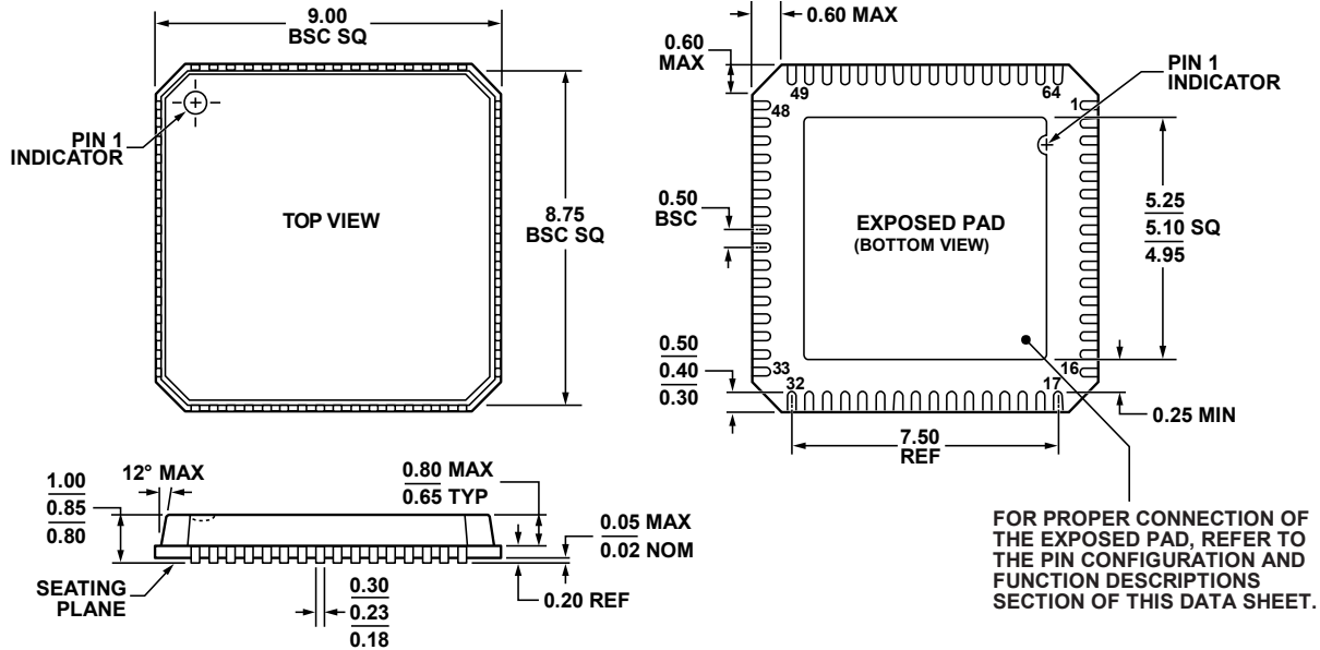
Figure 58. 64-Lead Lead Frame Chip Scale Package [LFCSP_VQ] 9 mm × 9 mm Body, Very Thin Quad (CP-64-5) Dimensions shown in millimeters
