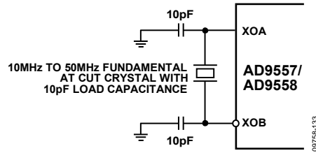
Figure 33. System Clock Input (XOA, XOB) in Crystal Mode (The recommended C_{LOAD} = 10\text{ pF} is shown. The values of the 10 pF shunt capacitors shown here should equal the C_{LOAD} of the crystal.)
