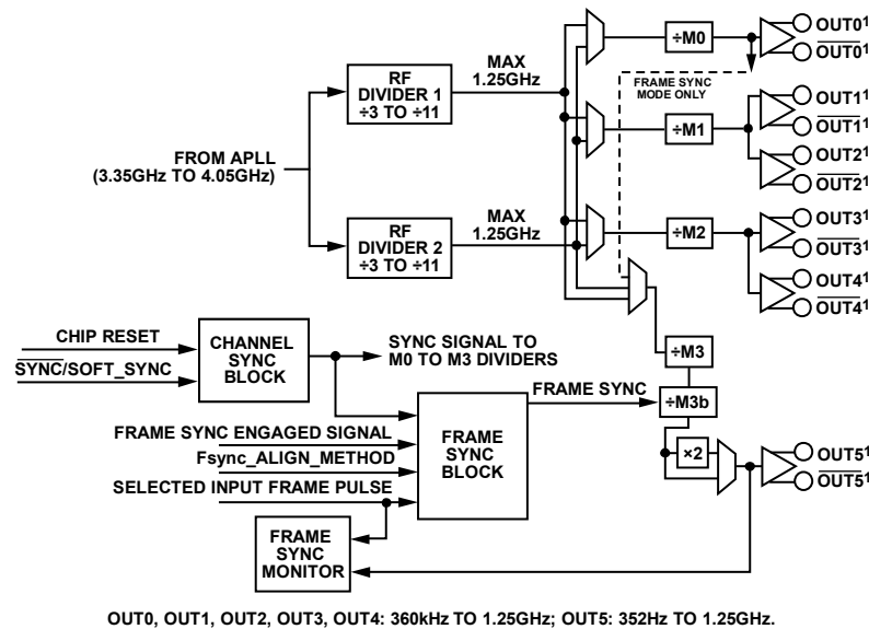
Figure 40. Clock Distribution Block Diagram
