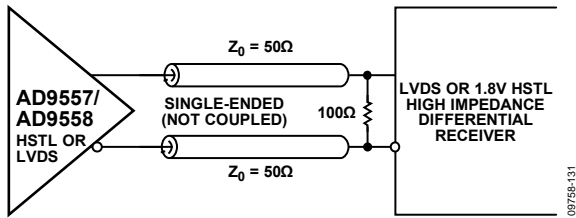
Figure 31. DC-Coupled LVDS or HSTL Output Driver
